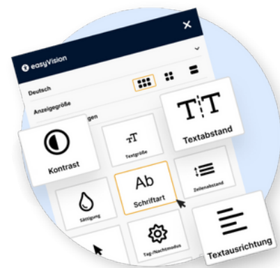
easyVision Widget 🔗
